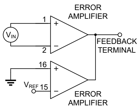
Fig. 2 AMPLIFIER CHARACTERISTICS
