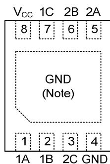
DFN2030-8 (Top View)
