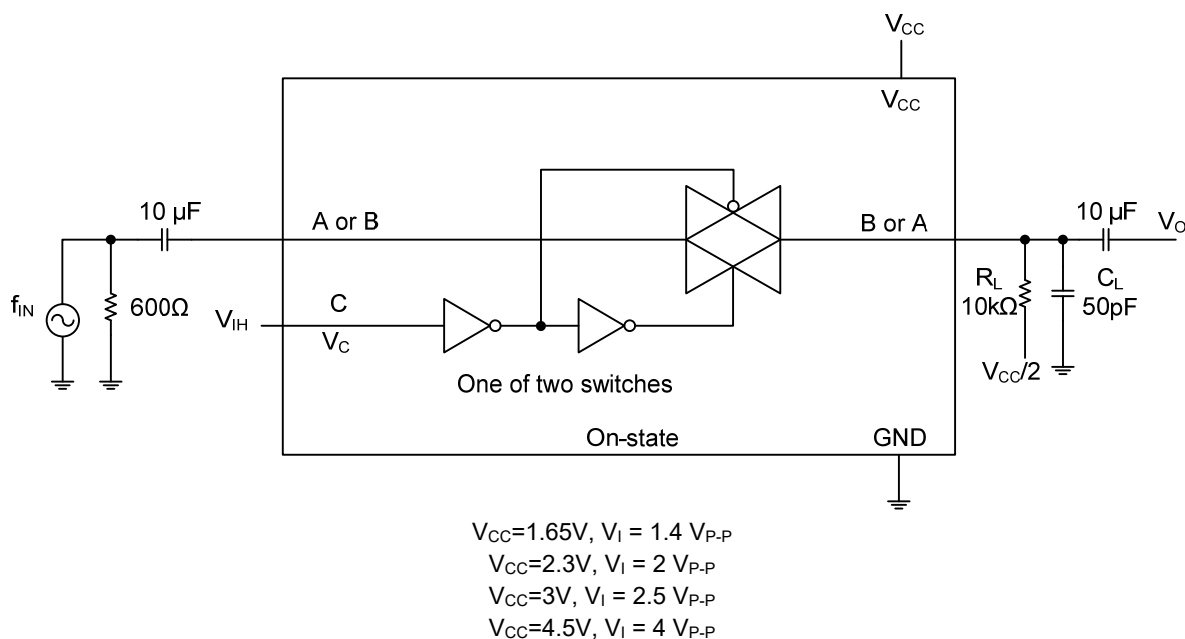
Fig.9 Sine-wave distortion
