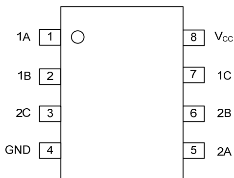
SOP-8/MSOP-8/TSSOP-8
