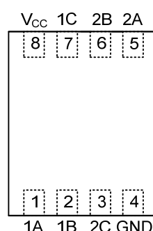
CDFN2030-8 (Top View)
