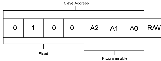
Figure 4. UCA9555 Device Address
