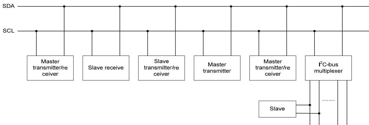
Figure 14. System configuration
