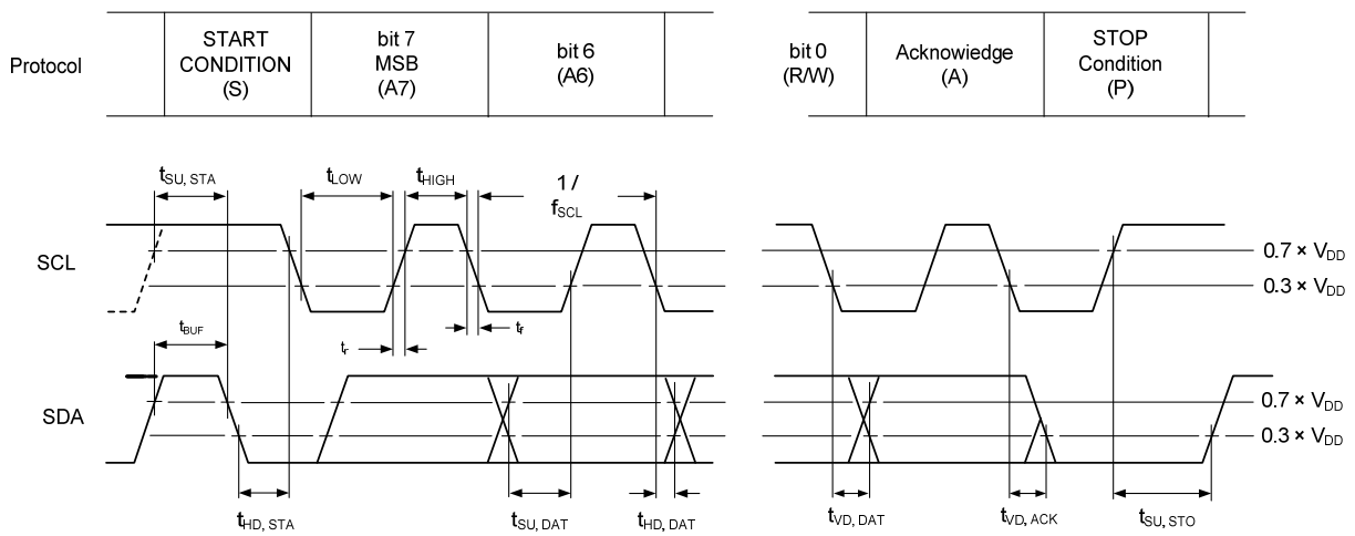
Figure 1. Definition of timing on the I 2 C-bus
