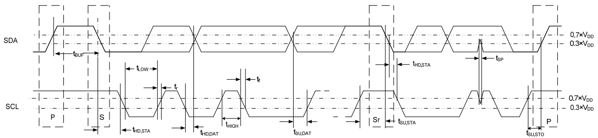
Figure 1. Definition of timing on the I 2 C-bus
