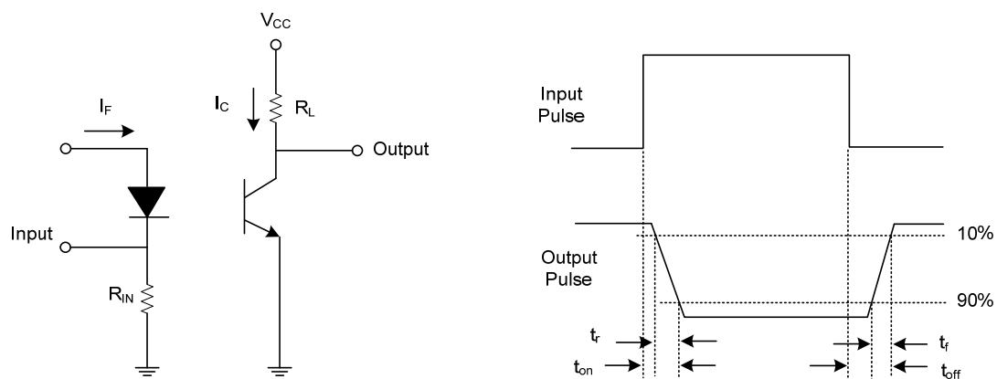
Switching Time Test Circuit &amp; Waveforms
